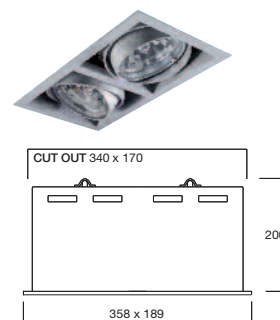
DFD2150/C/EL/L Framelight 2
