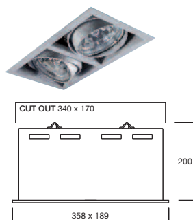
DFD2035/C/EL/L Framelight 2
