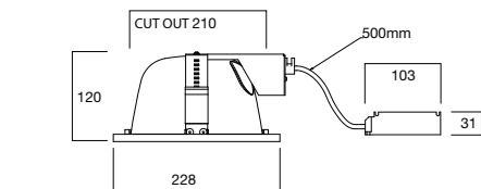
(a) D88 Series: TC-DEL Compact Fluorescent
