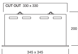
DFAD4070/C/EL/L24 Framelight 4
