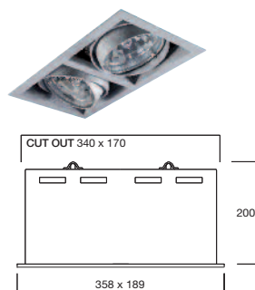
DFD2070/C/EL/L Framelight 2
