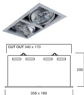
DFAD2070/C/EL/L24 Framelight 2
