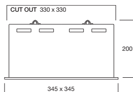
DFD4035/C/EL/L Framelight 4
