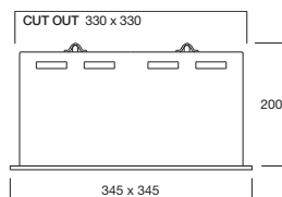
DFD4070/C/EL/L Framelight 4
