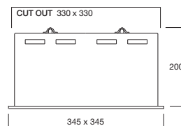
DFD4150/C/EL/L Framelight 4
