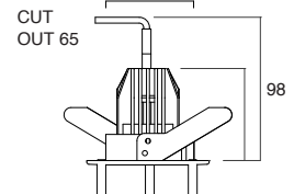
LED Open with Disc Glass
