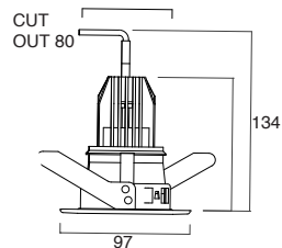
LED Black baffle
