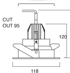
LED Silver Cone
