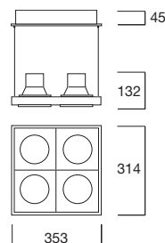
DFDS2X24035/C/EL/L Framelight 2 x 2 way Suspended SG ■
