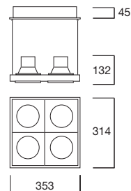
DFDS2X24070/C/EL/L Framelight 2 x 2 way Suspended SG ■
