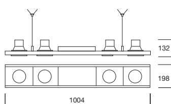
DFDS4035/C/EL/L Framelight 4 way Suspended SG ■
