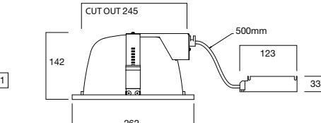
(b) D98 Series: TC-TEL Compact Fluorescent
