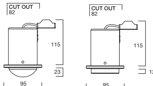
Interchangeable Domed Glass / Flat Glass
